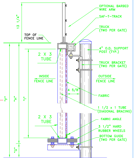
END VIEW AT SUPPORT POST SCG-TO 24 FT.DWG
